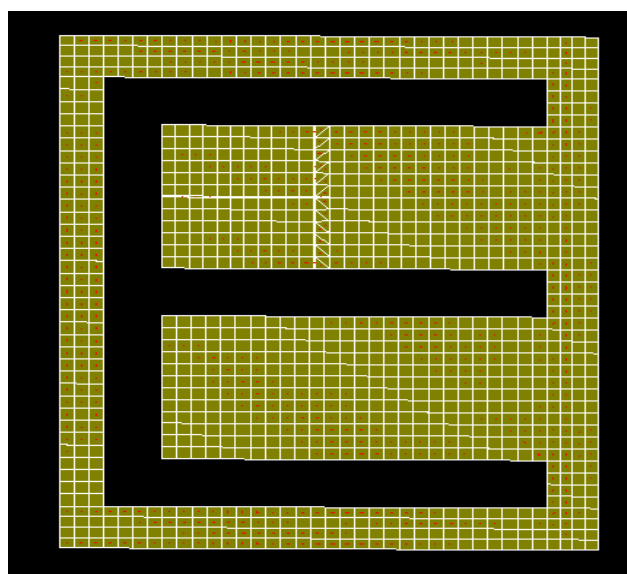
Fig.2: Simulated E-shaped antenna current distributions
